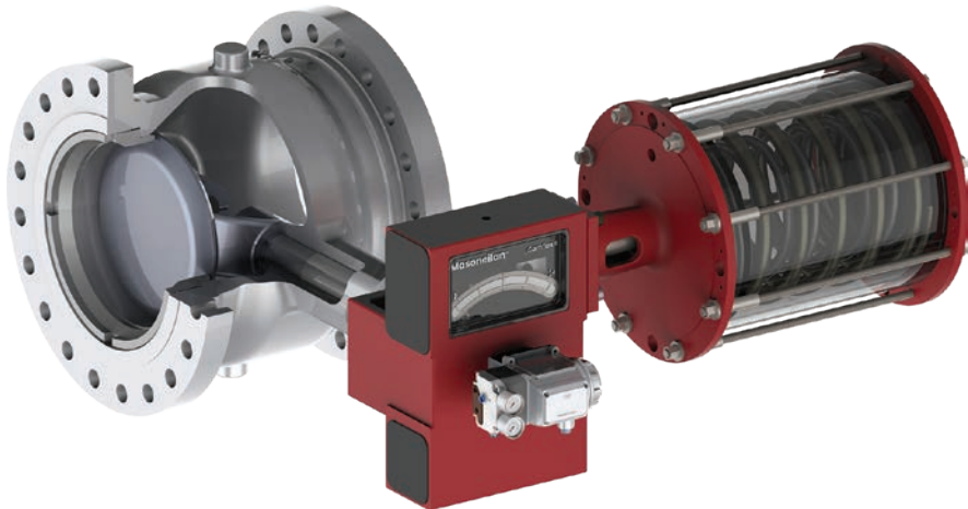
Camflex High Capacity Design – sectional view
