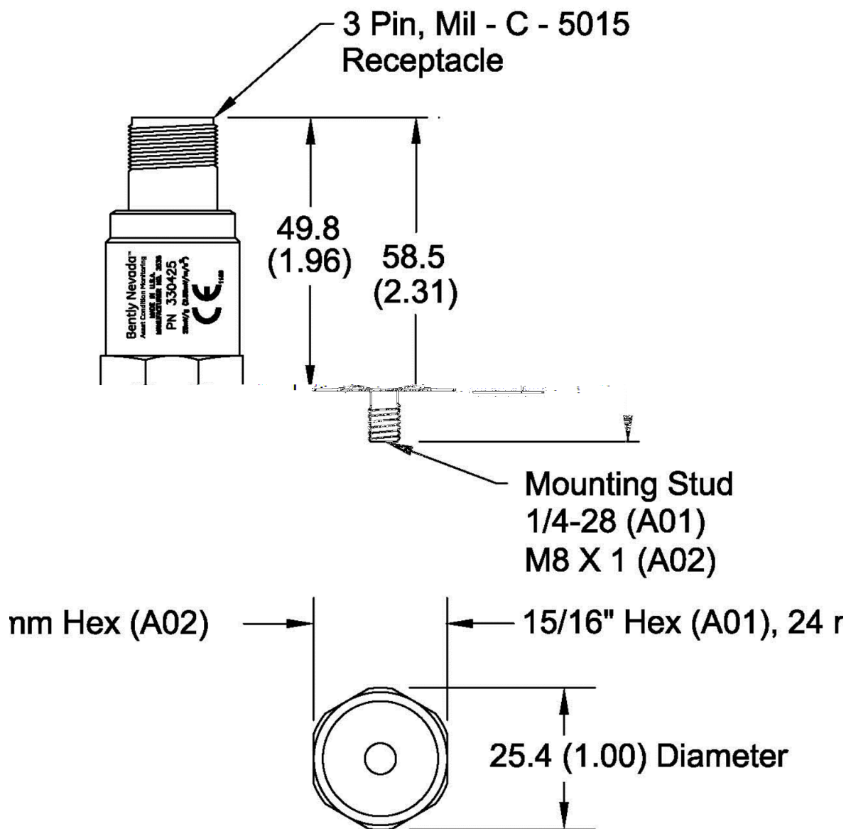
Figure 1: Acceleration Transducer Dimensional Drawing
